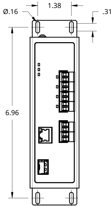
WALL MOUNT
