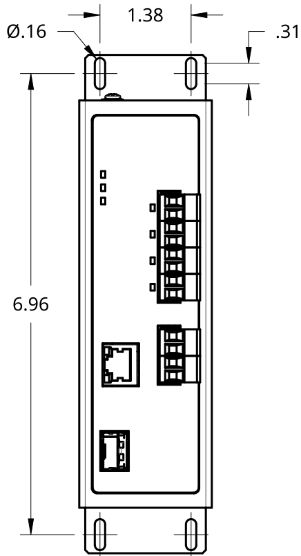
WALL MOUNT
