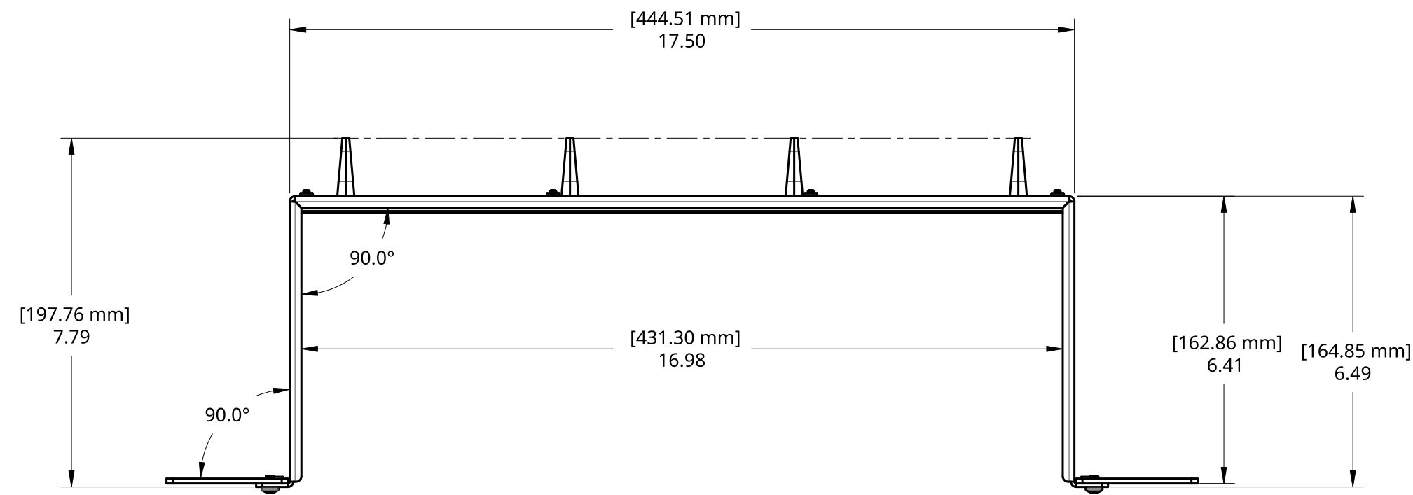
TOP VIEW
