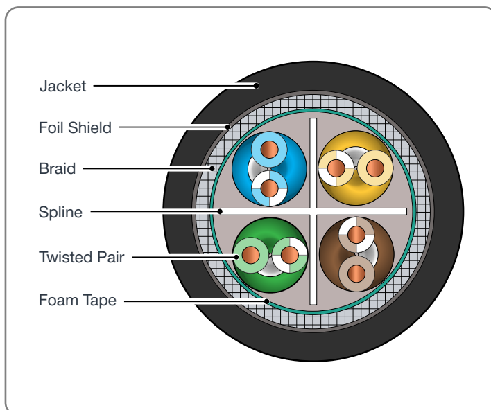
Cross Section
