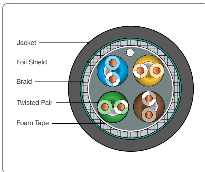
Cross Section
