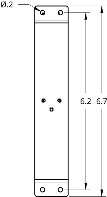
WALL MOUNT
