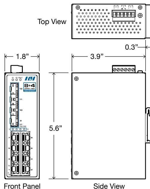
Dimensional Information
