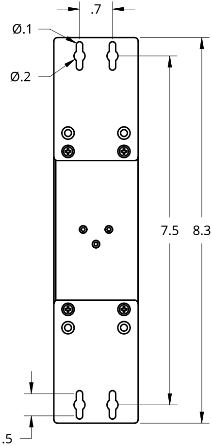
WALL MOUNT
