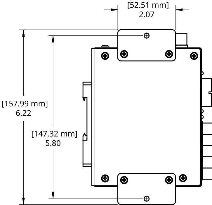
LEFT VIEW
