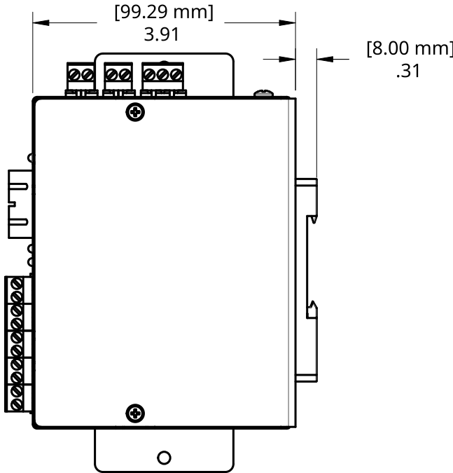
RIGHT VIEW
