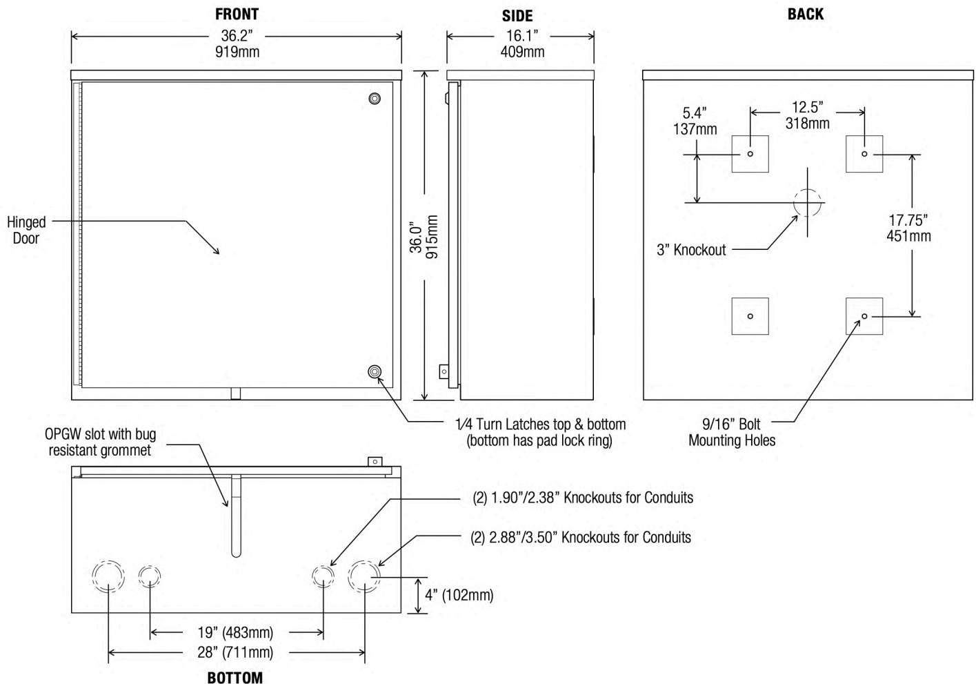
Splice Cabinet Exterior Dimensions
