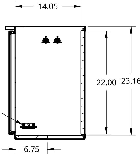
SECTION A - A INTERNAL DETAIL
