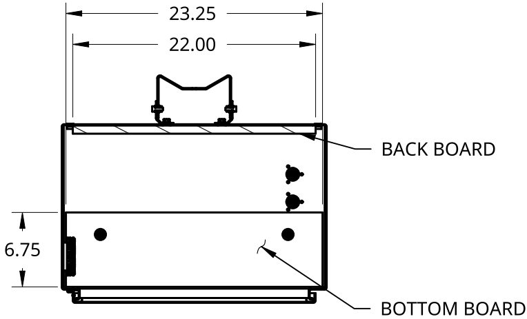
SECTION B - B INTERNAL DETAIL
