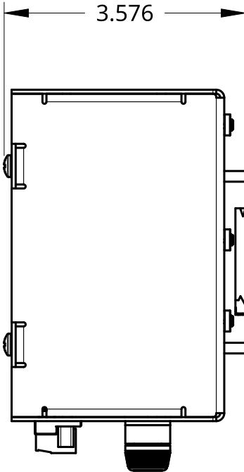
RIGHT VIEW
