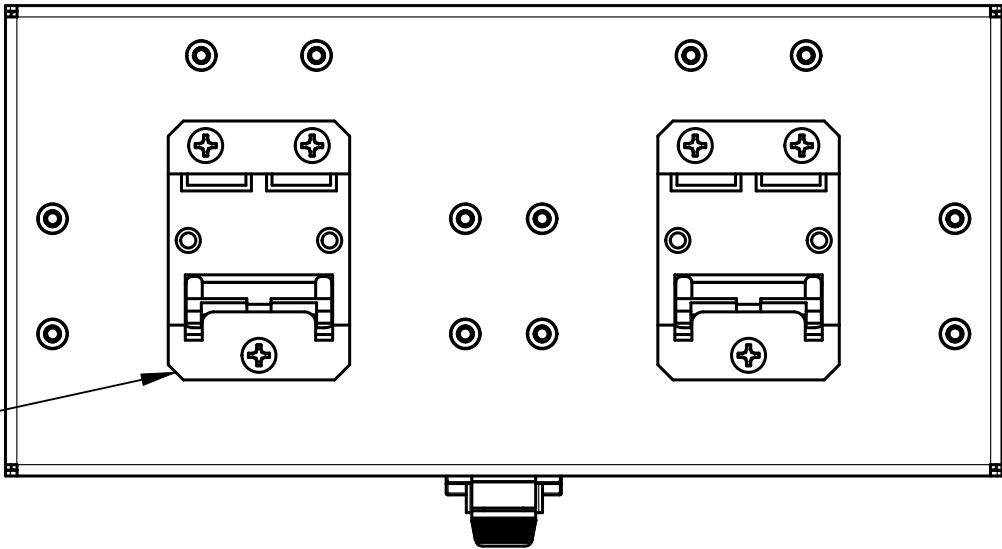
BACK VIEW
