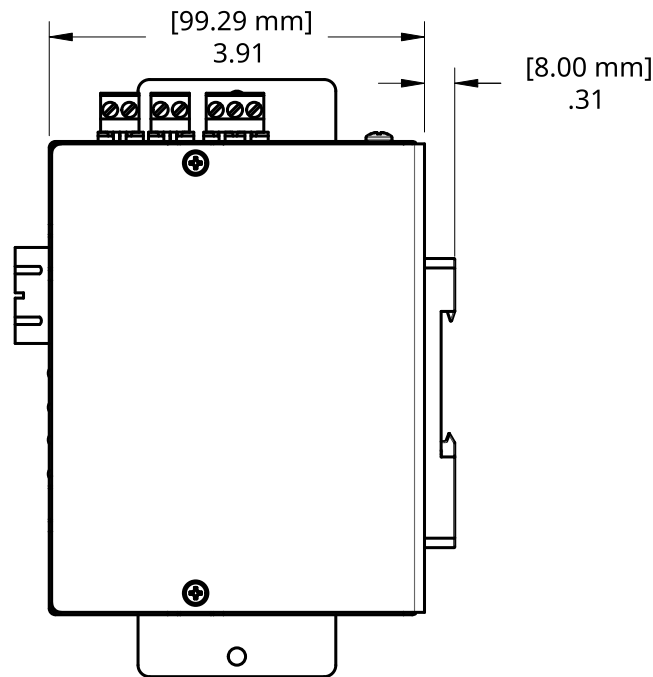
RIGHT VIEW
