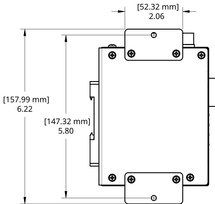
LEFT VIEW
