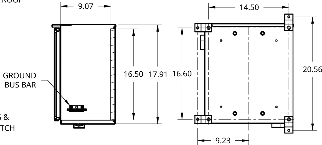
SECTION A - A INTERNAL DETAIL
