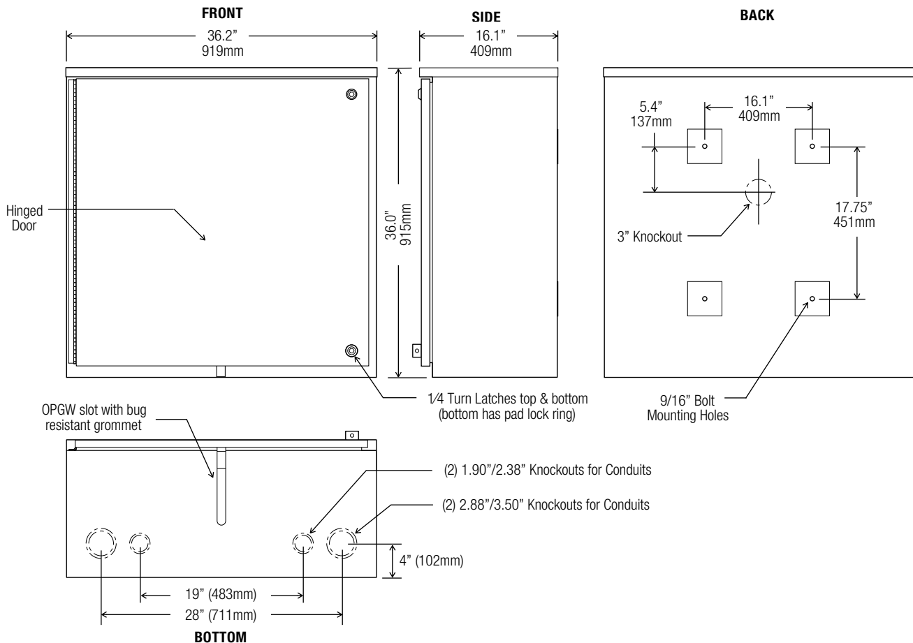
Splice Cabinet Exterior Dimensions
