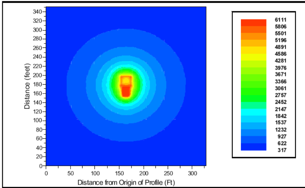
Figure 7. GPR Profile (North is Up)
