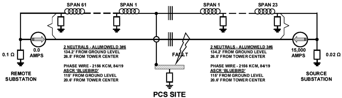
Figure 5. Fault Grounding Schematic
