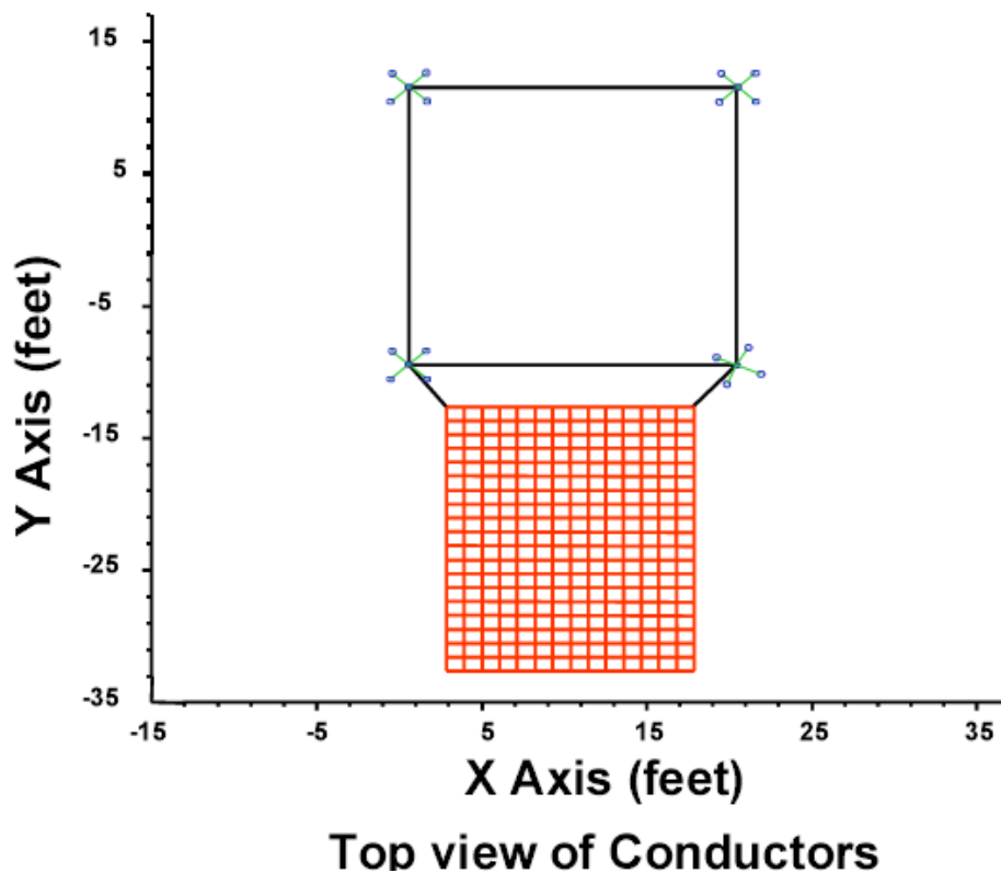
Figure 4. Layout of Site Grounding Modeled
