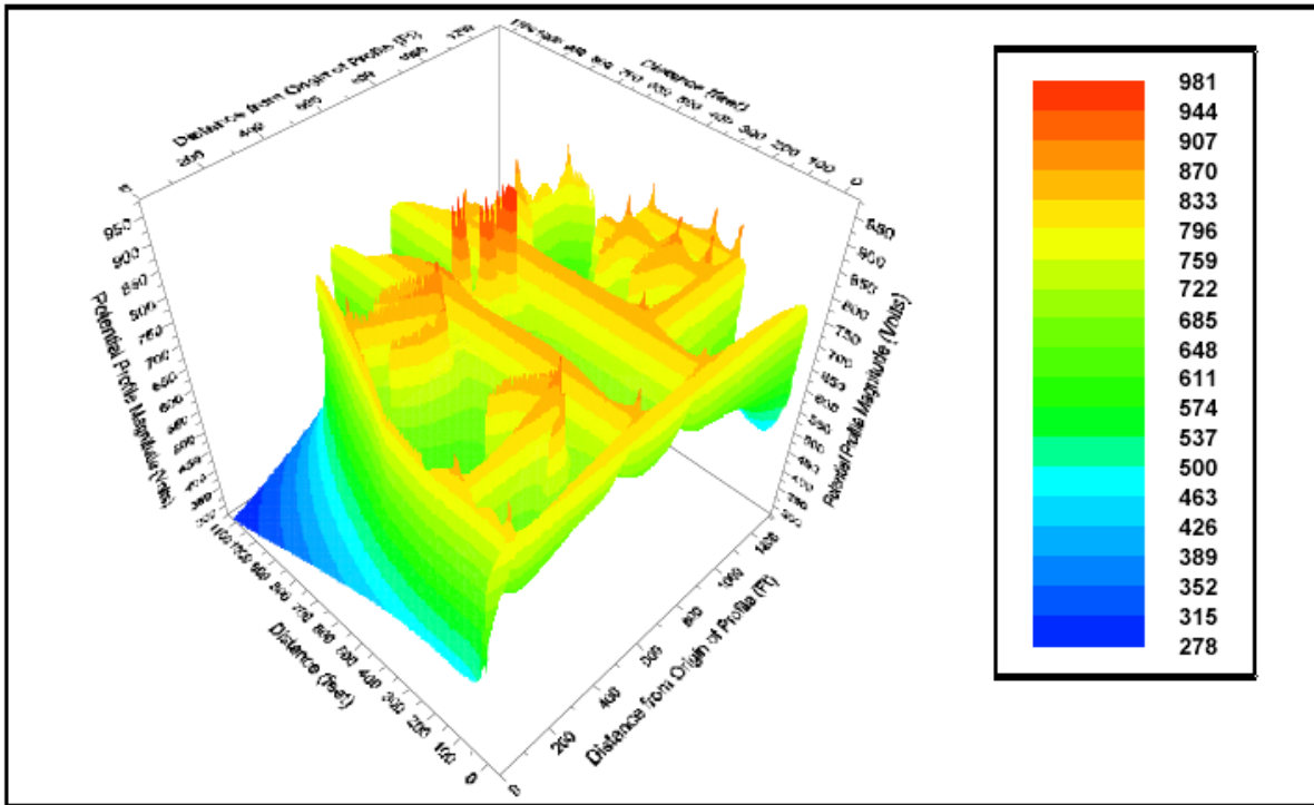
Figure A2. GPR Profile with Limited MGN Connections Identified
