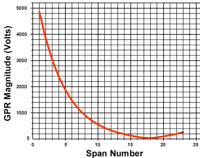
Figure 6. GPR (Shunt Potential) for each HV tower back to the SOURCE substation
