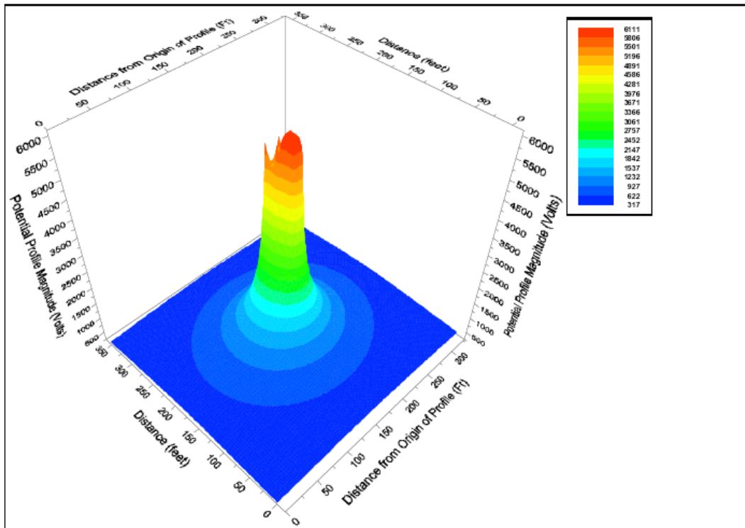
Figure 8. GPR Profile in 3-D
