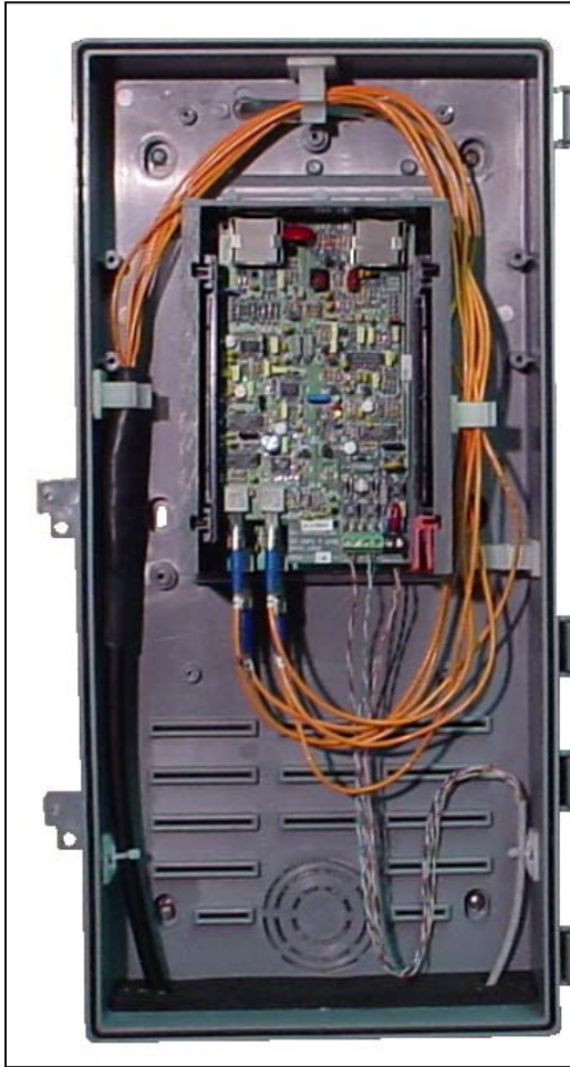
Figure 1 Four-Card Suggested Wiring and Fiber Routing
