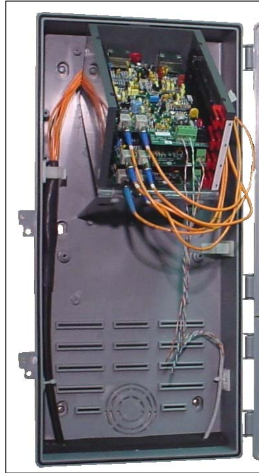
Figure 2 Four-Card Swing-Out for Testing and Maintenance
