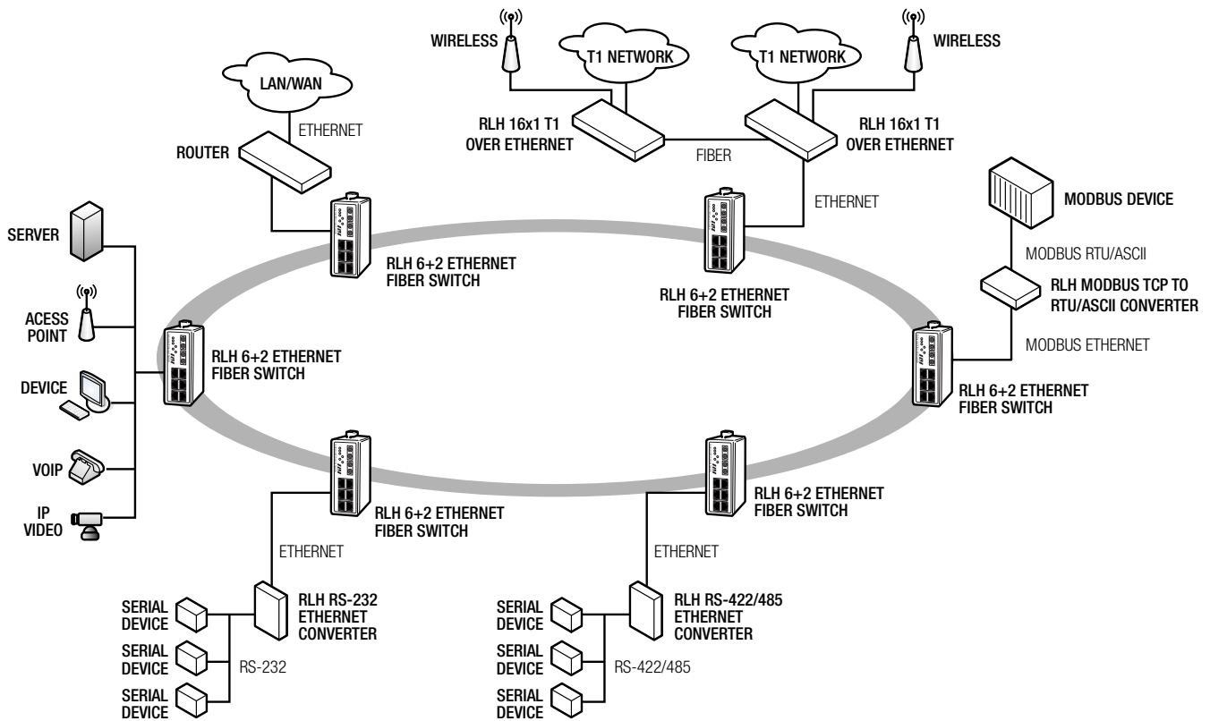
Redundant Ring Fiber Network Topology
