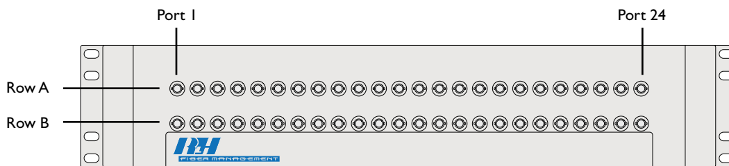
48 Port ST/ST Rack Mount Fiber Optic Patch Panel Front View
