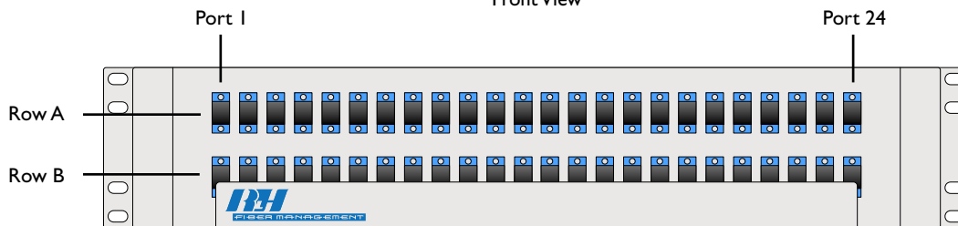
48 Port SC/SC Rack Mount Fiber Optic Patch Panel Front View
