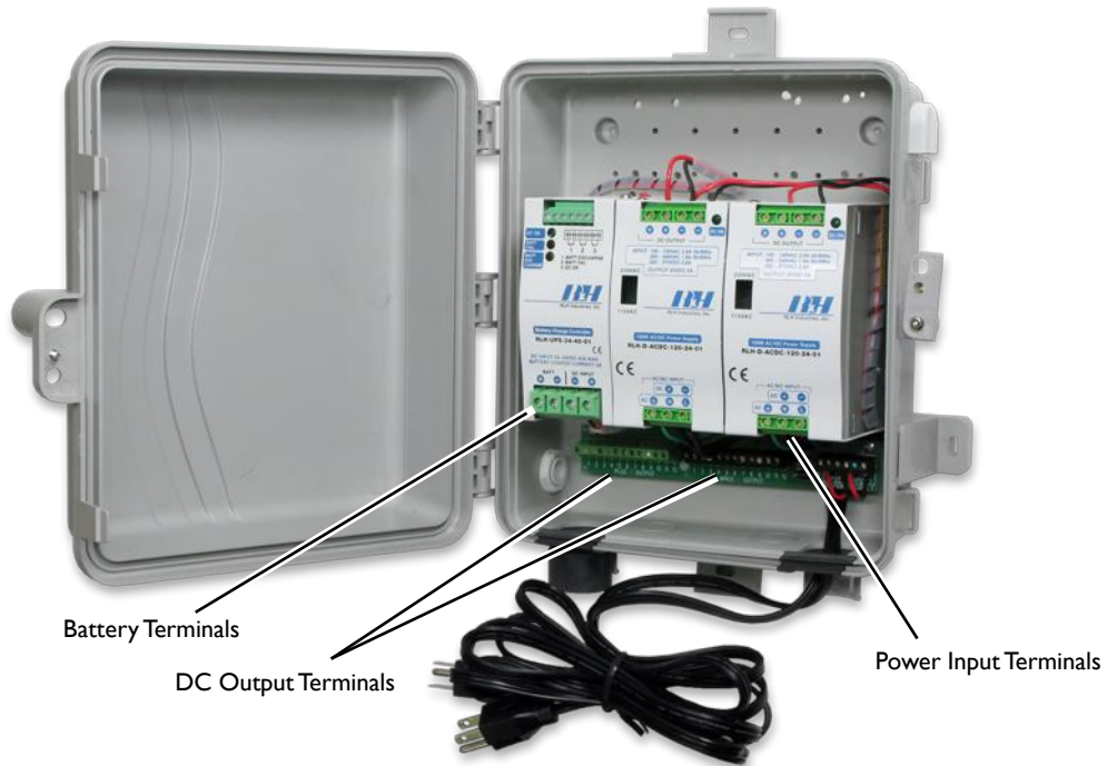
Internal Components - Redundant power supply model shown
