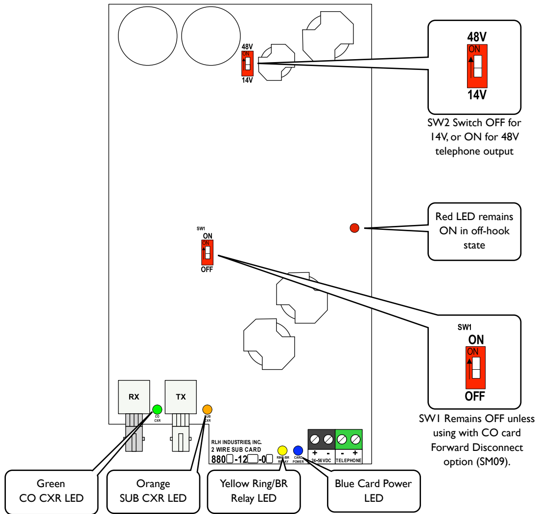
FXS/Sub LED indicators and switches
