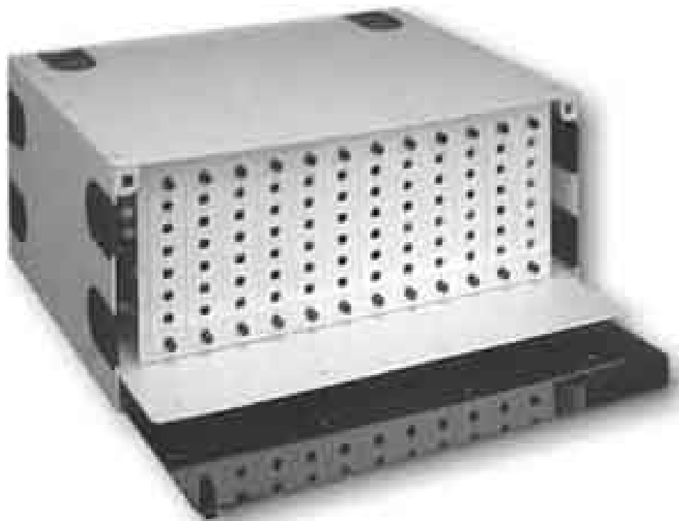
RLH-72RST-01 Rack Mount Enclosure/Patch Panel with ST Connectors for 72 Fibers Dimensions: 7.25"H x 17.25"W x 13.25"D Weight: 19 Pounds
